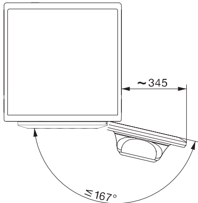
WT1 8/5 kg, drawing, straight fascia, measures in mm
